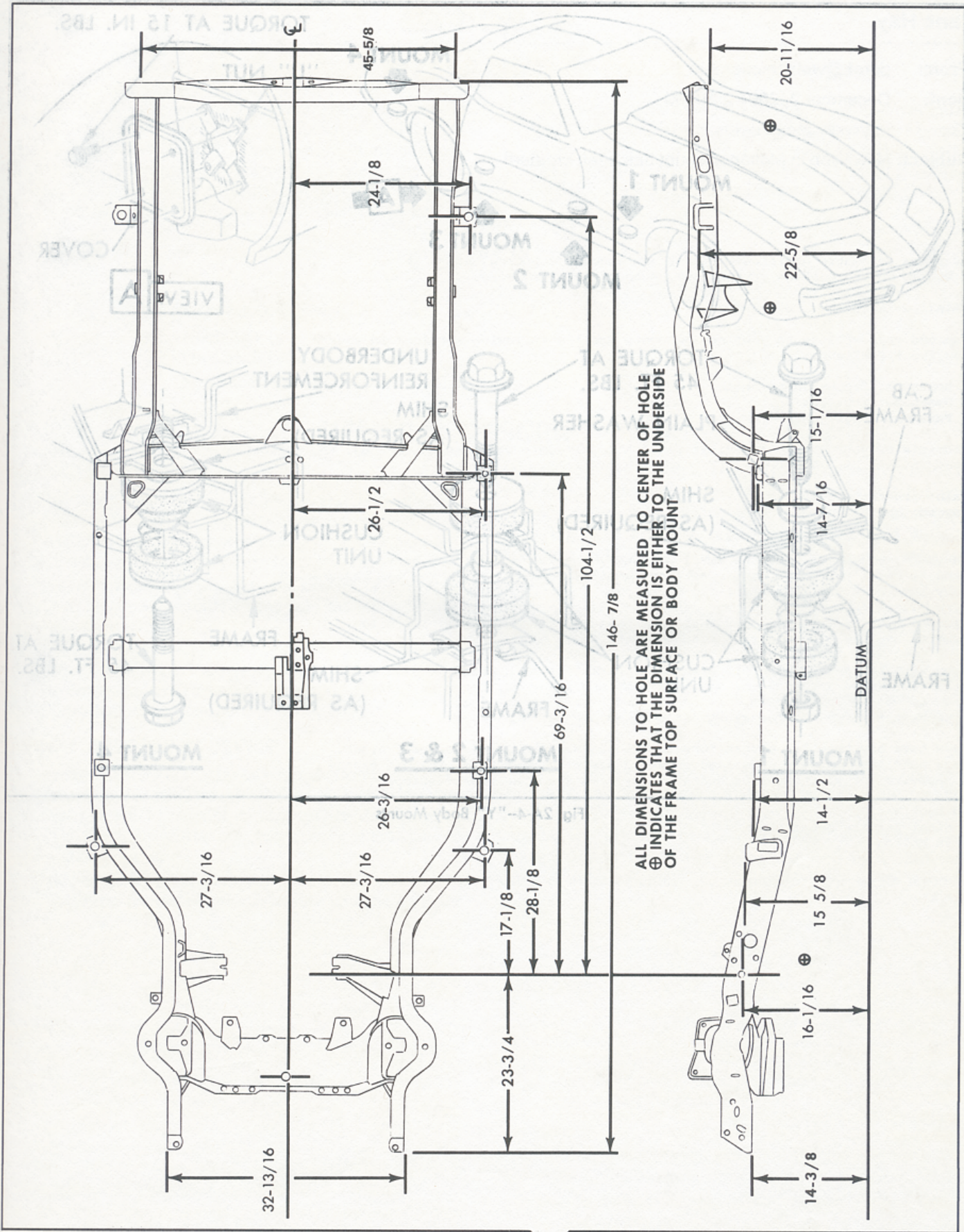
Fig. 2A-3--Corvette Frame Dimensions
