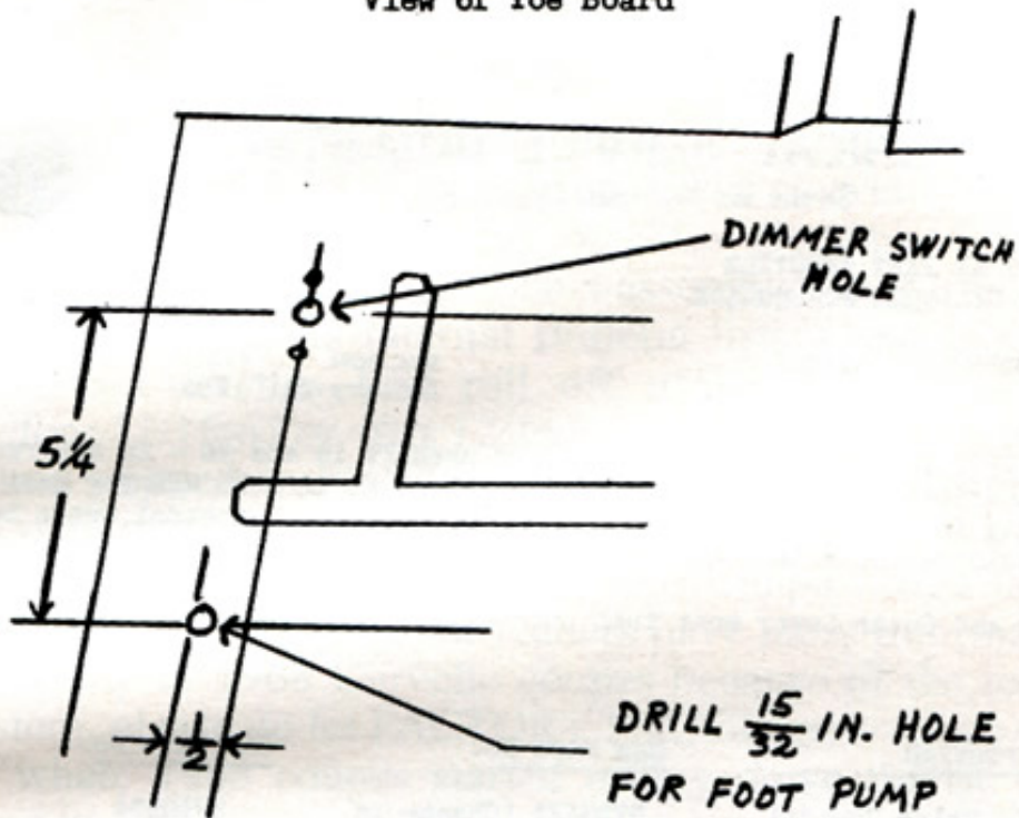
View of Toe Board
