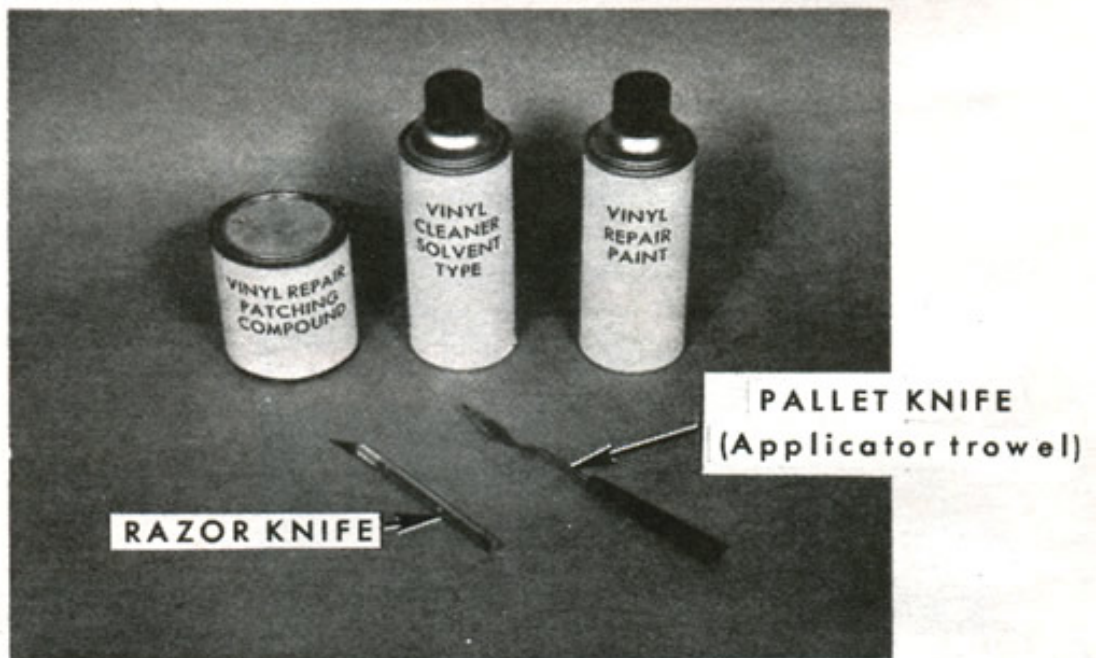
FABRIC ROOF COVER REPAIR MATERIALS AND TOOLS
