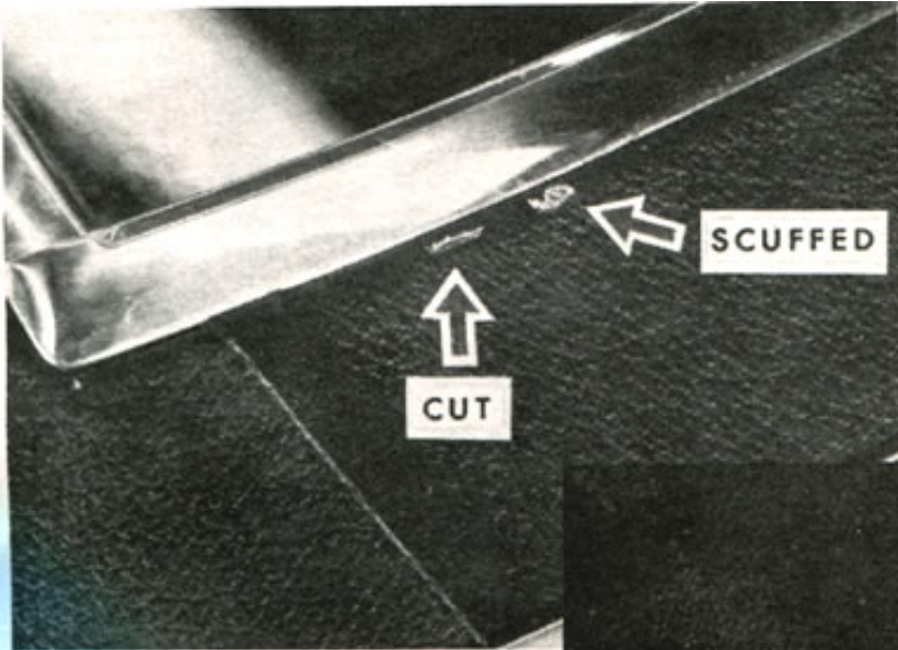
TYPICAL FABRIC ROOF COVER DIS- CREPANCIES FIGURE 1
