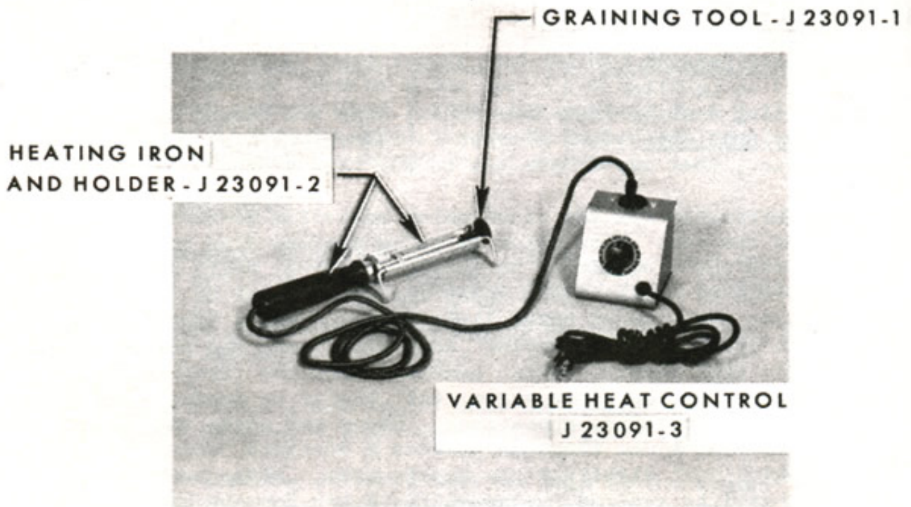
FABRIC ROOF COVER TOOL - TOOL J 23091 (Consist of three pieces)
