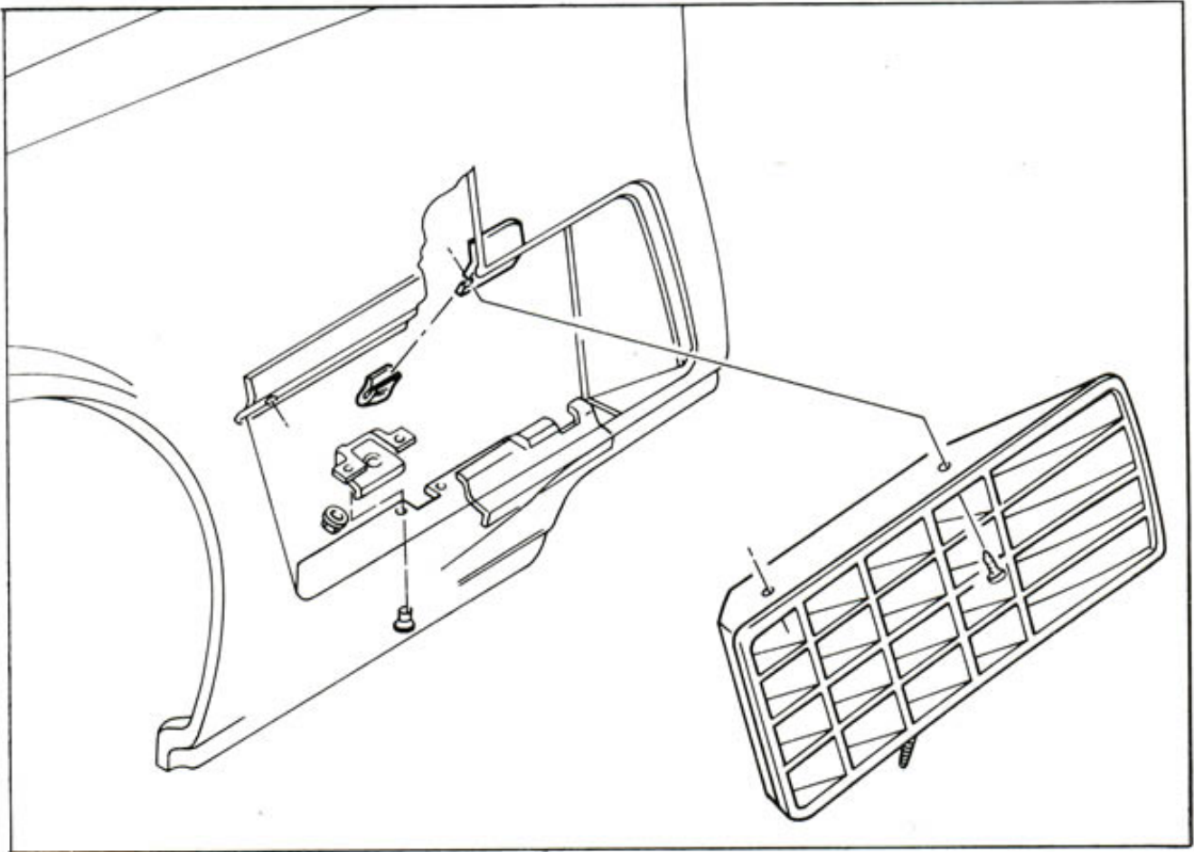
Figure 1—Fender Side Louver
