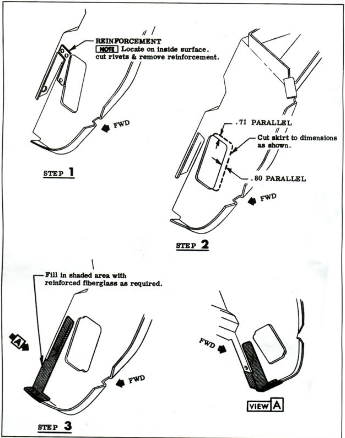
Fig. 2—Corvette Fender Rework
