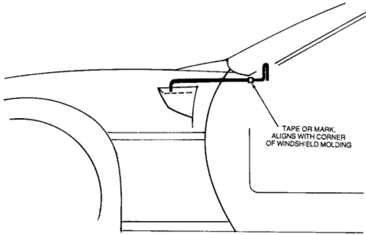
TOOL IN POSITION (DOOR REMOVED FOR ILLUSTRATIVE PURPOSES)
