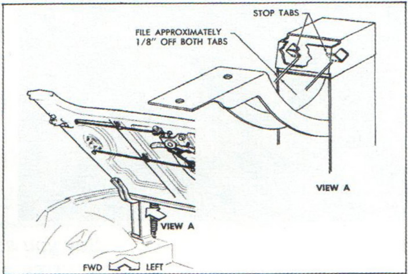
Fig. 12—Remove \frac{1}{8} " From Lid Stops
