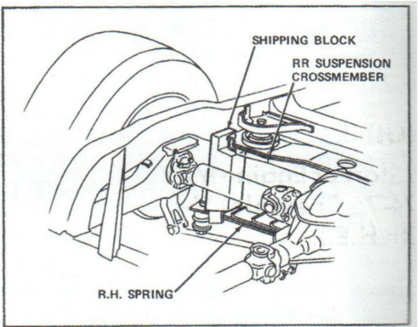
Fig. 1—Shipping Block Location
