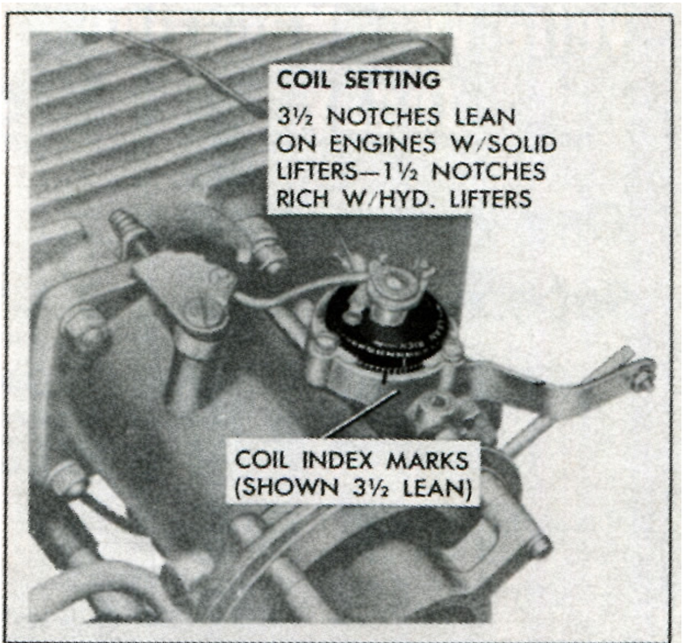
Fig. 2—Fuel Injection Cold Enrichment
