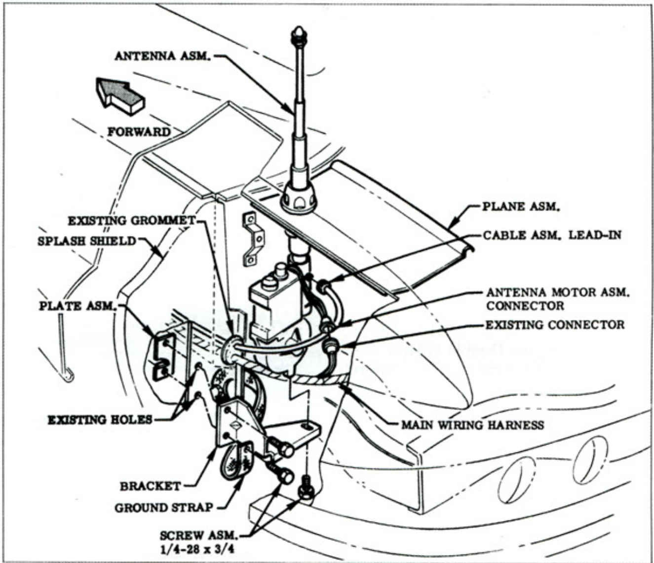
Fig. 2—Corvette Power Operated Rear Antenna
